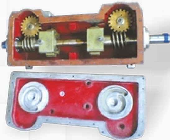
screen drive gear box assembly
