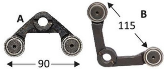
screen guide bearing bracket 90mm & 115mm center
